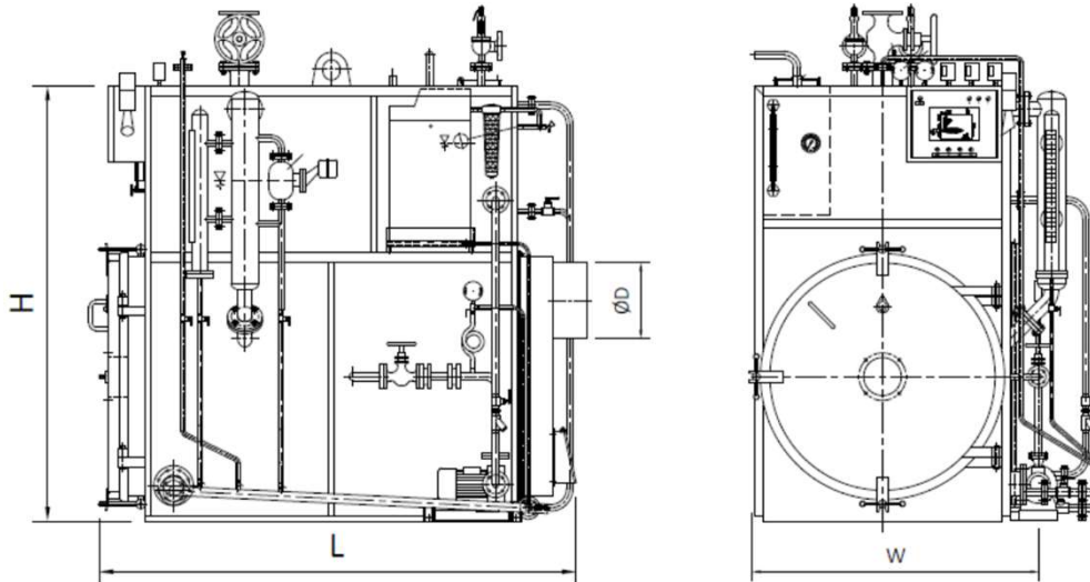
ESG SERIES STEAM GENERATOR PRELIMINARY DIMENSIONS
